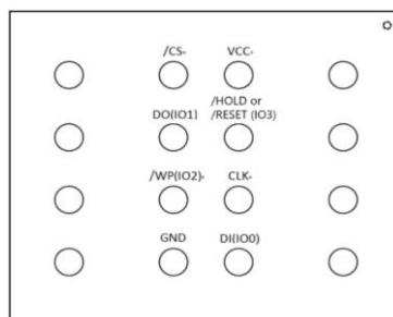
Figure 1d. DS25M4AE Pad Assignments, 16Ball WLCSP (Bottom View)
