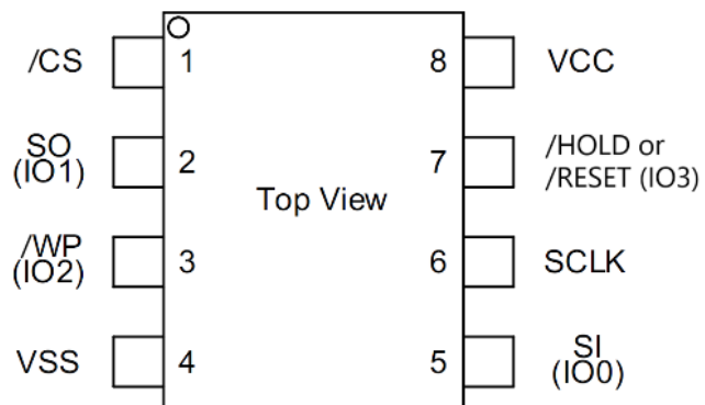
Figure 1a. 8-pin SOP 208-mil
