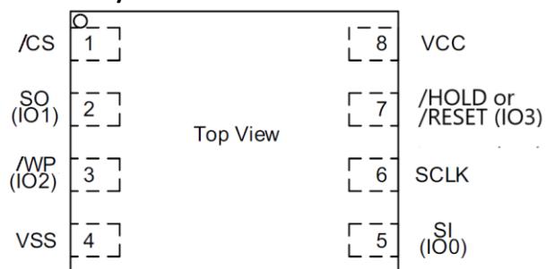
Figure 1c. 8-pad WSON 6x5-mm
