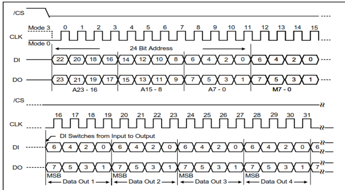
Figure 14b. Fast Read Dual I/O Instruction (Previous instruction set M5-4 = 10, SPI Mode only, 4 Dummy)
