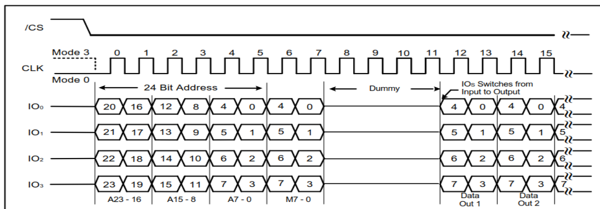
Figure 15b. Fast Read Quad I/O Instruction (Previous instruction set M5-4 = 10, SPI Mode, 6 Dummy)
