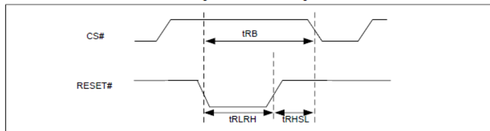
Figure 50. Reset Timing
