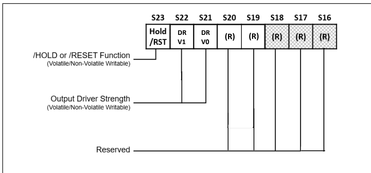
Figure 4c. Status Register-3
