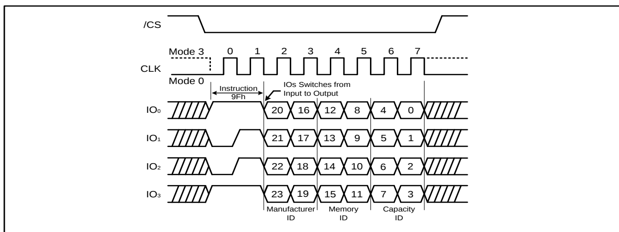
Figure 34b. Read JEDEC ID Instruction (QPI Mode)
