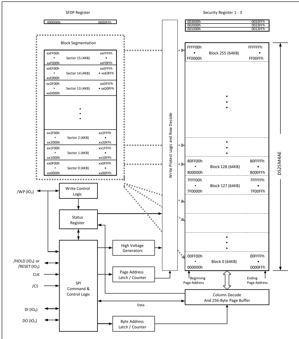
Figure 2. DS25M4AE Serial Flash Memory Block Diagram
