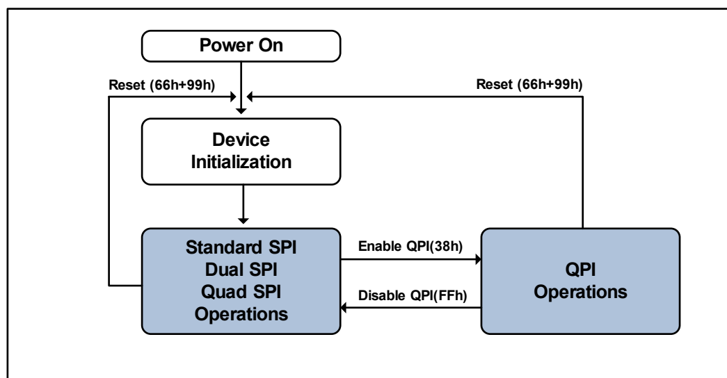
Figure 3. DS25M4AE Serial Flash Memory Operation Diagram
