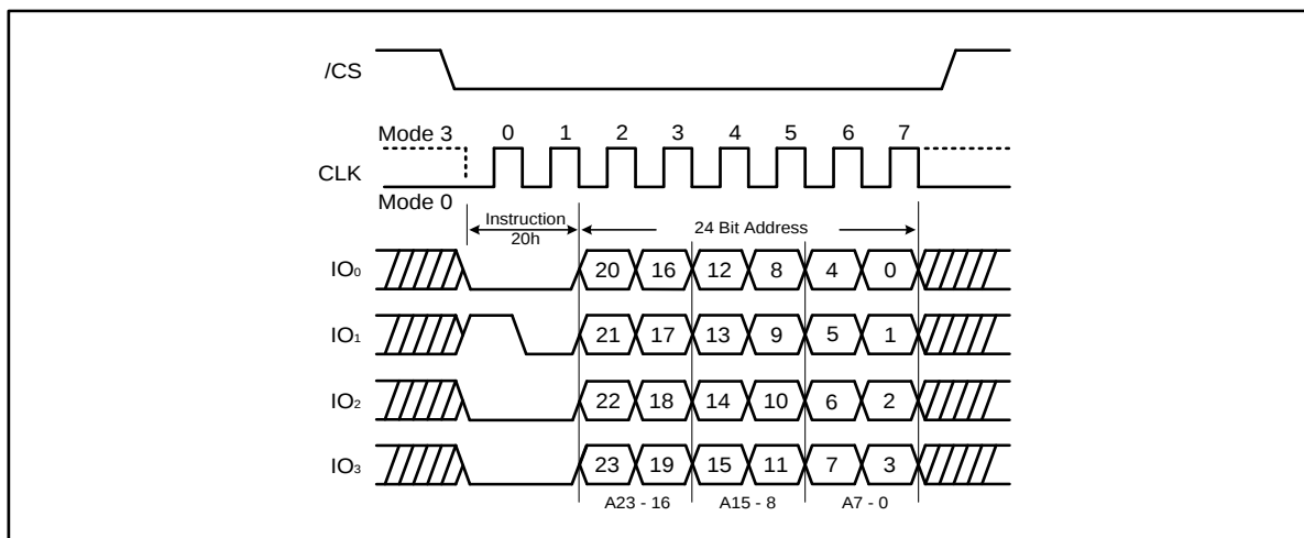
Figure 22b. Sector Erase Instruction (QPI Mode)
