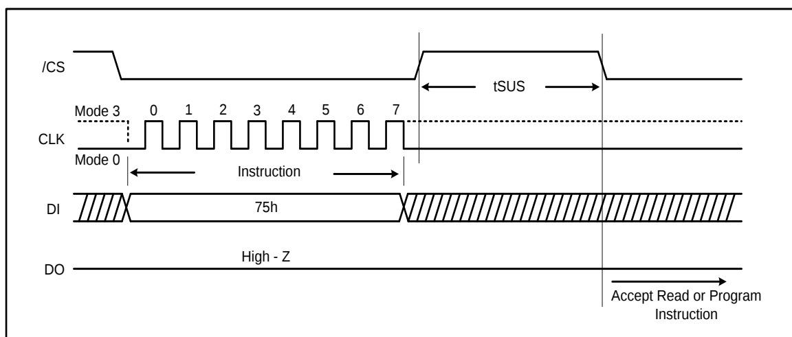
Figure 26a. Erase/Program Suspend Instruction (SPI Mode)
