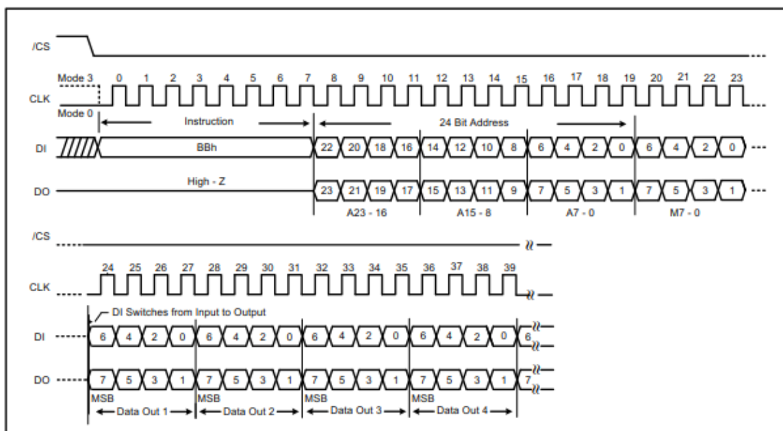
Figure 14a. Fast Read Dual I/O Instruction (Initial instruction or previous M5-4 ≠ 10, SPI Mode only, 4 Dummy)
