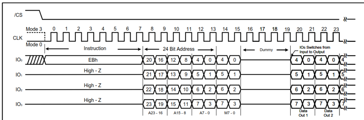
Figure 15a. Fast Read Quad I/O Instruction (Initial instruction or previous M5-4 ≠ 10, SPI Mode, 6 Dummy)
