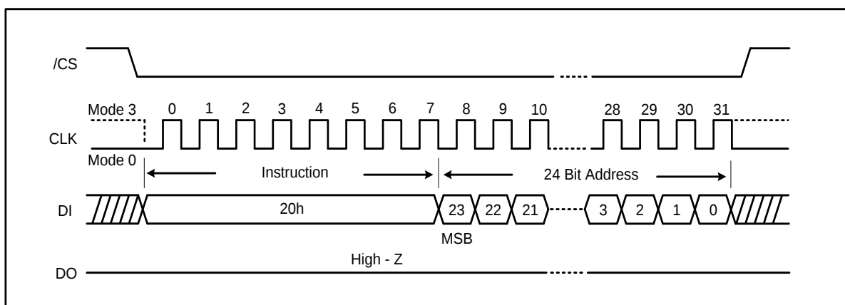
Figure 22a. Sector Erase Instruction (SPI Mode)
