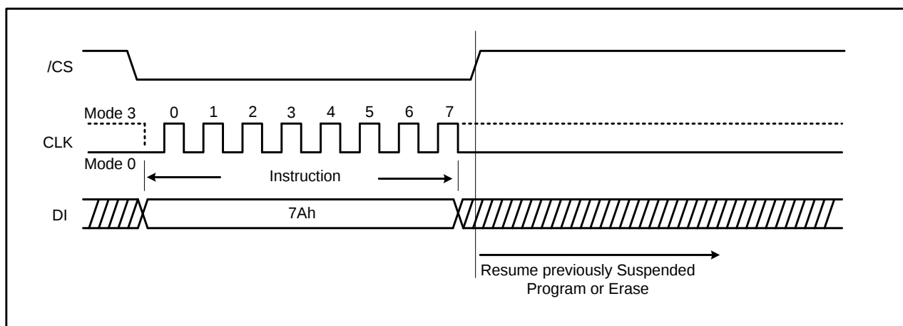
Figure 27a. Erase/Program Resume Instruction (SPI Mode)
