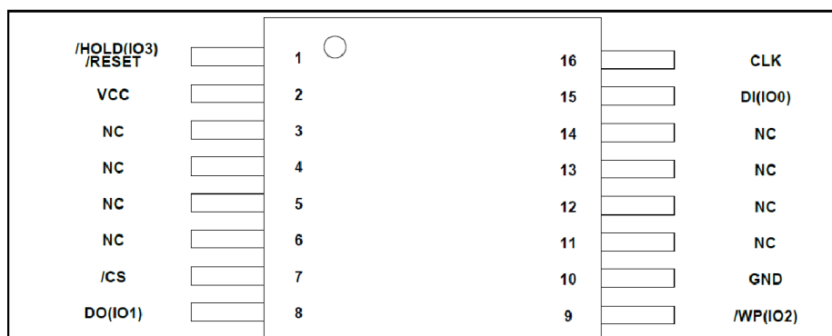
Figure 1b. 16-pin SOP 300-mil
